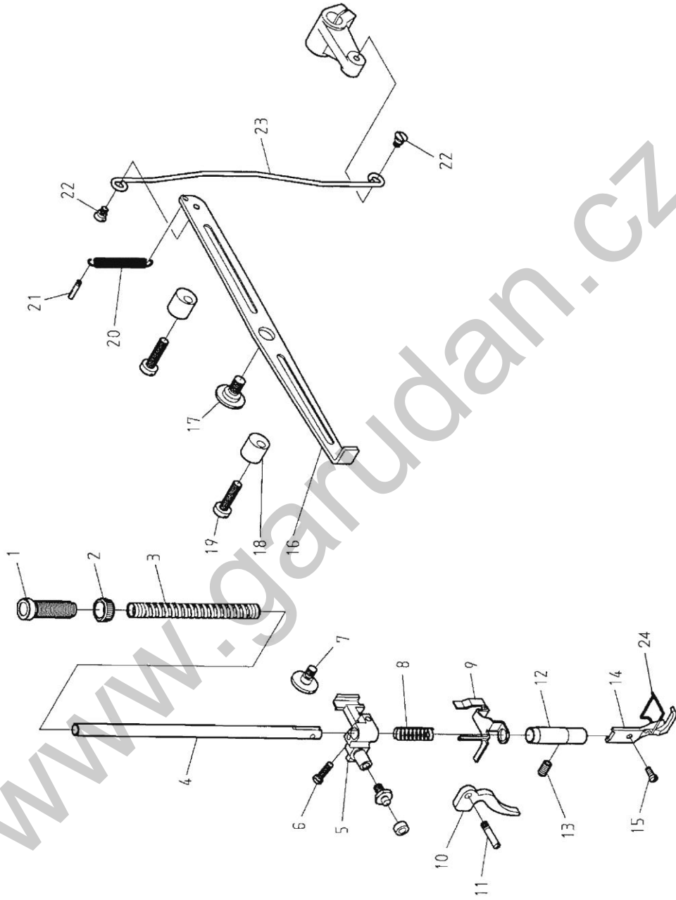
F. PRESSURE BAR & KNEE LIFTER COMPONENTS (1/3)
